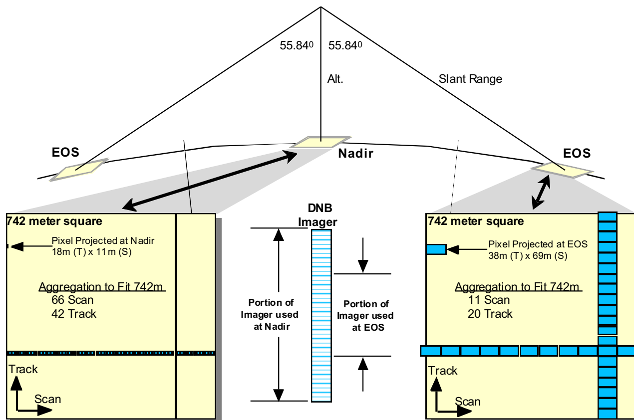
Figure 2.2-5: VIIRS DNB Sub-pixel Aggregation
