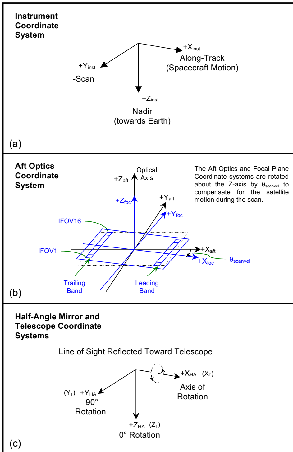
Figure 3.3-3: Instrument, Aft Optics and Half Angle Mirror Coordinate Systems' Relative Orientation
