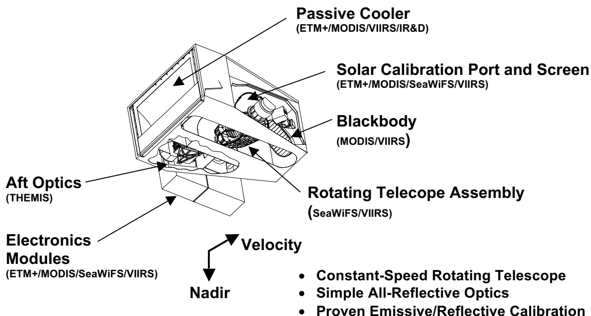
Figure 2.2-1: Summary of VIIRS Design Concepts and Heritage
