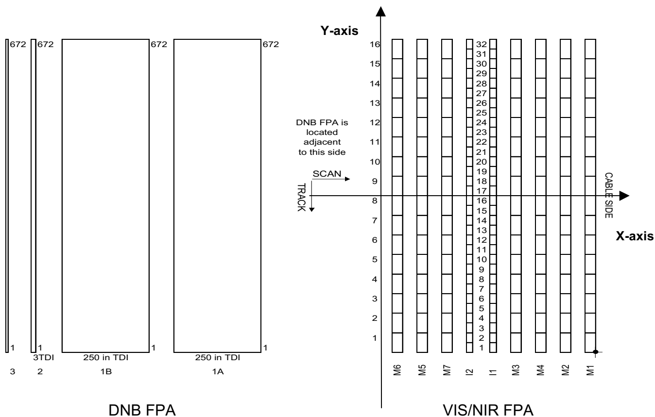
Figure 3.3-2A: CCD and Detector Layout (DNB and VIS/NIR)
