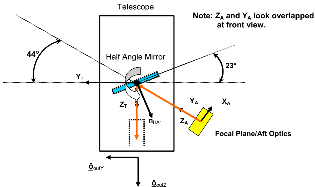
Figure 3.3-4: Off-Nadir View, Half Angle Mirror Rotation, Telescope Rotation in Instrument Coordinate System
