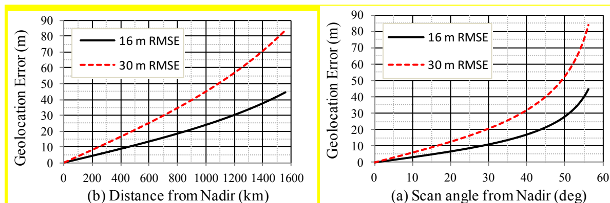
Figure 3.4-8: Geolocation Error resulting from various Terrain Height Errors as a Function of (a) Scan Angle and (b) Distance from Nadir.
