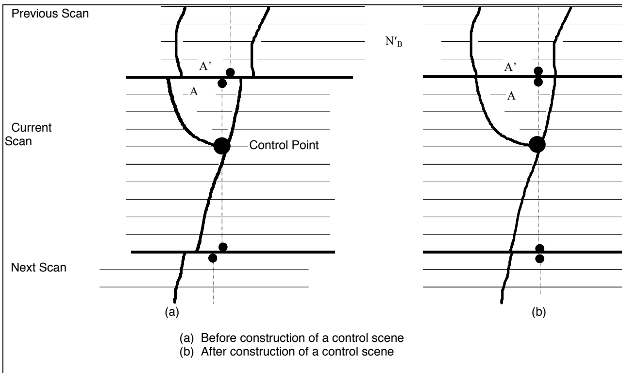
Figure 3.4-9: Connecting Parts of 3 Scans
